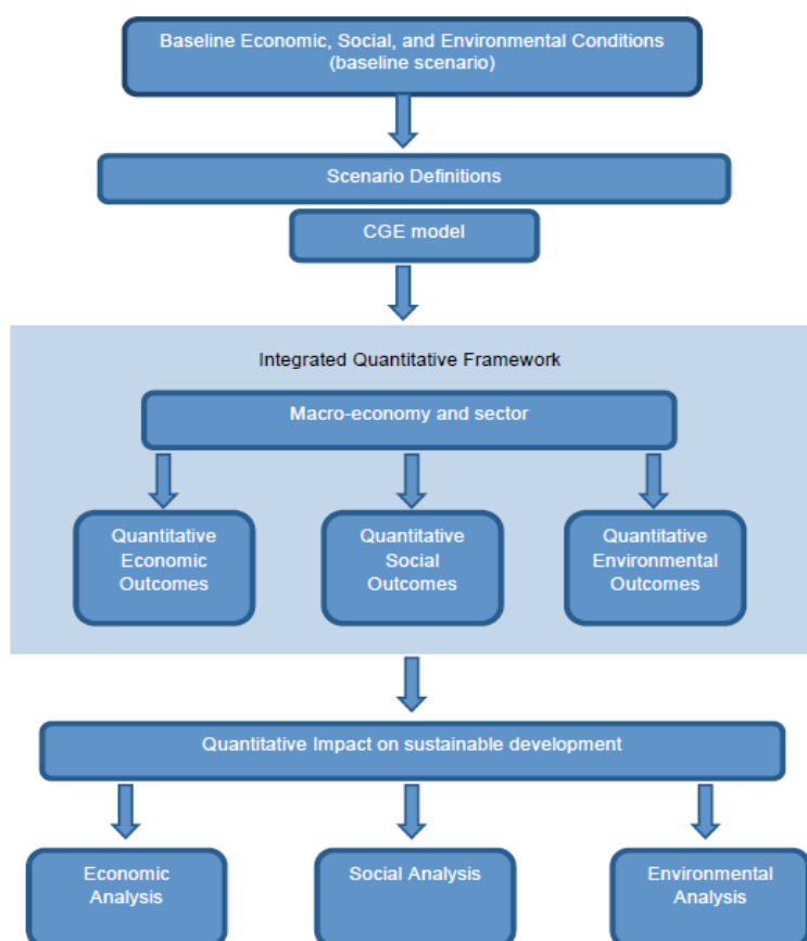
Figure 1.2 CGE methodology
